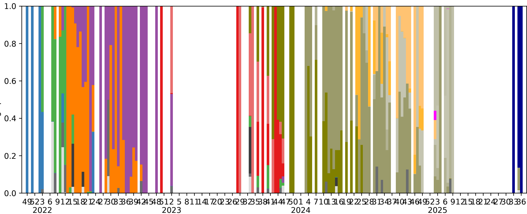
Lineage prevalence
